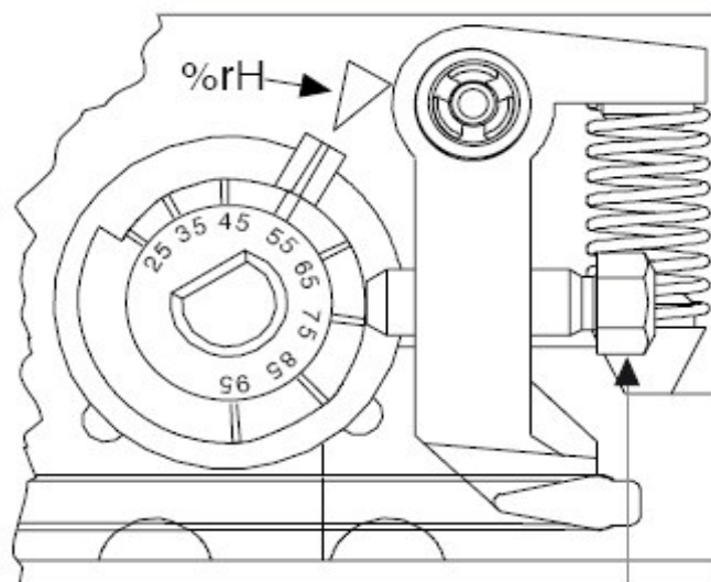
Calibrating screw (varnish-locked)
